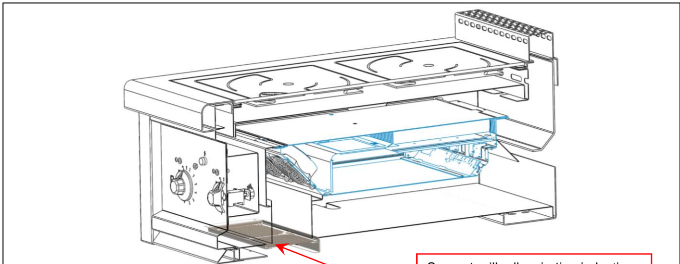
Support grille d'aspiration induction
